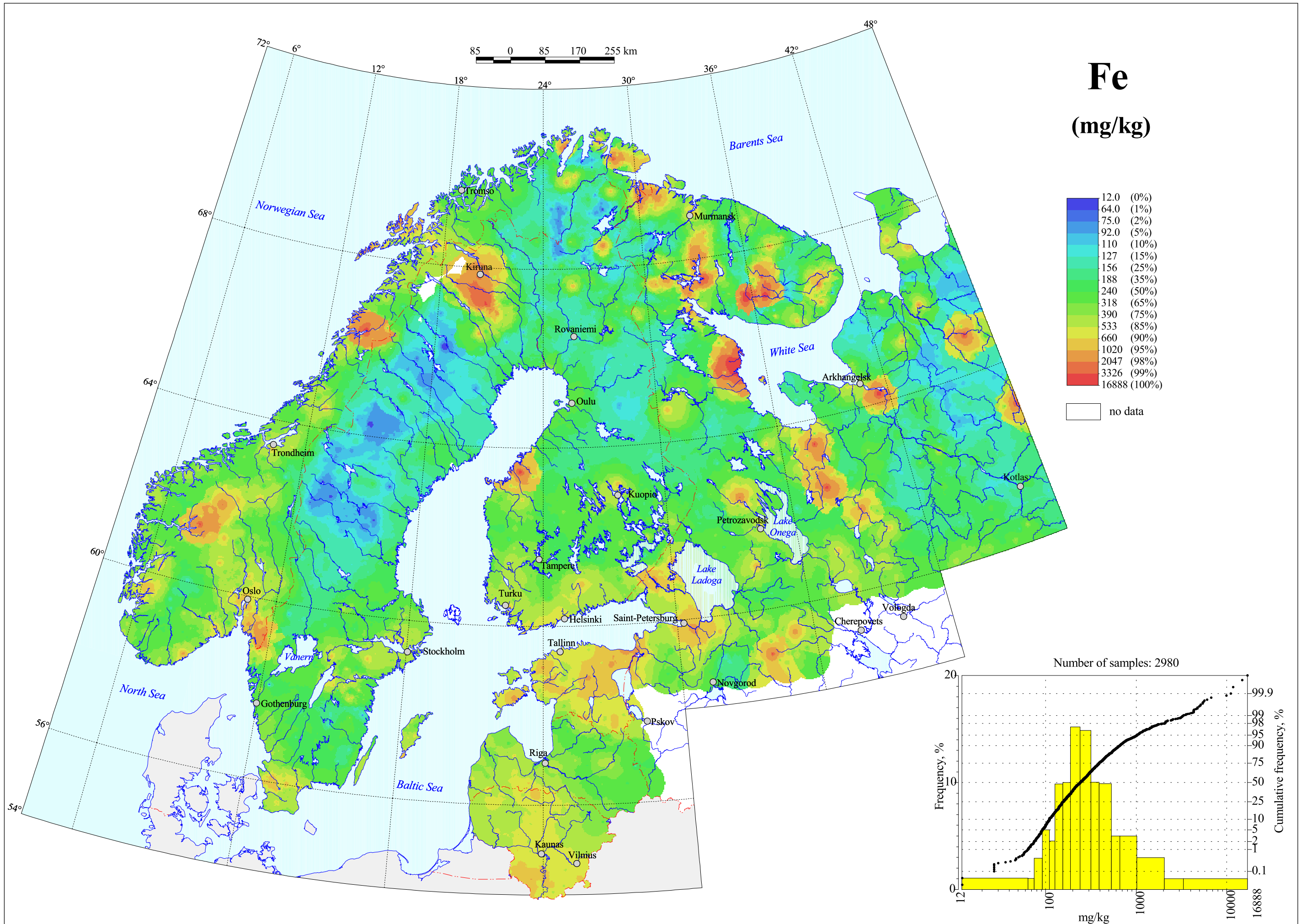
Iron in Terrestrial Moss, Total Content
